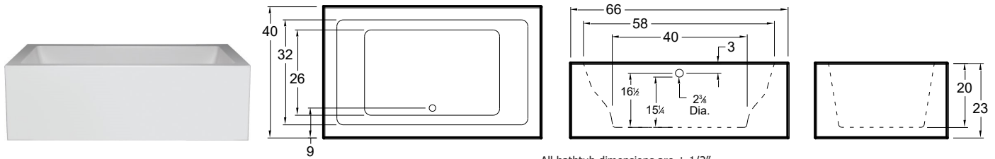
All bathtub dimensions are ± 1/2"
